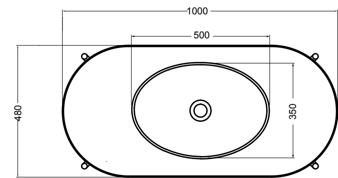
200M madia ovale 100x48x35 cm_oval sideboard 100x48x35 cm 200R ripiano_shelf 200S4507 struttura per madia ovale h 45 cm_frame for oval sideboard h 45 cm
