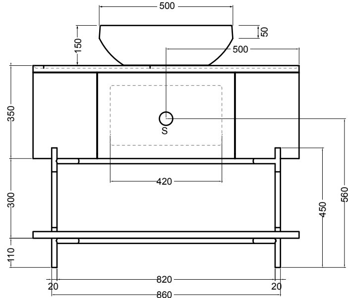
VISTA FRONTALE FRONT VIEW
