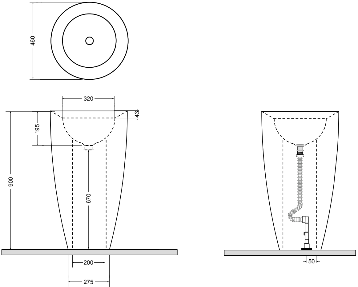
83400 lavabo freestanding suolo_freestanding basin floor
