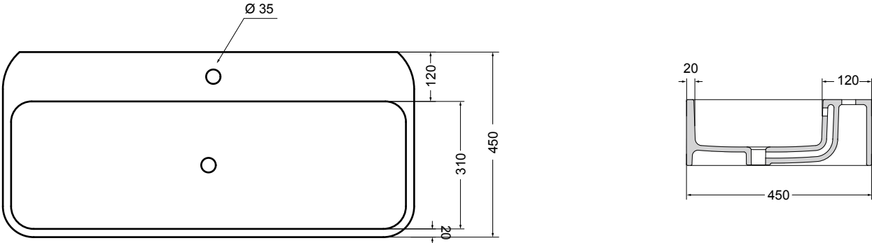
86400 lavabo appoggio/sospeso 100x45 cm_counter-top/wall-hung basin 100x45 cm
