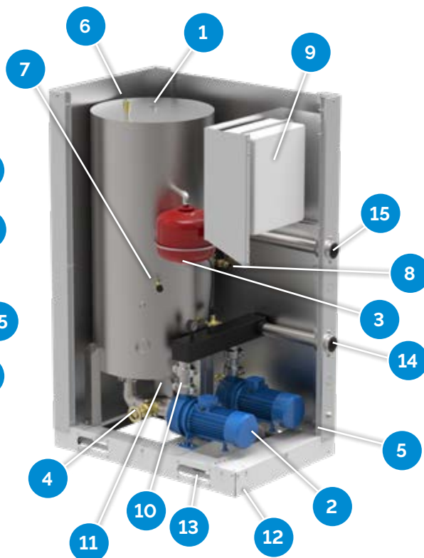
HPT Verticale
