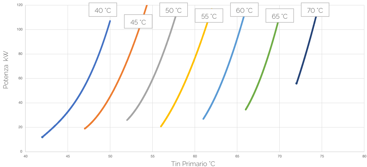
AQUAFAST 25/100 \Delta T=20^{\circ}\text{C}
