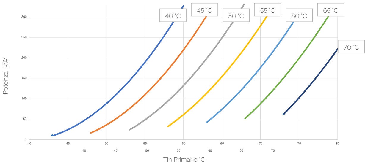
AQUAFAST 80/350 \Delta T=20^{\circ}\text{C}
