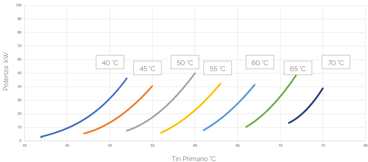
AQUAFAST 12/35 \Delta T=20^{\circ}\text{C}
