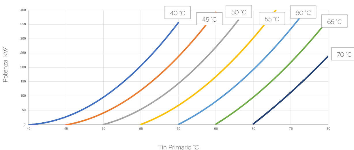
AQUAFAST 80/350 \Delta T=20^{\circ}\text{C}
