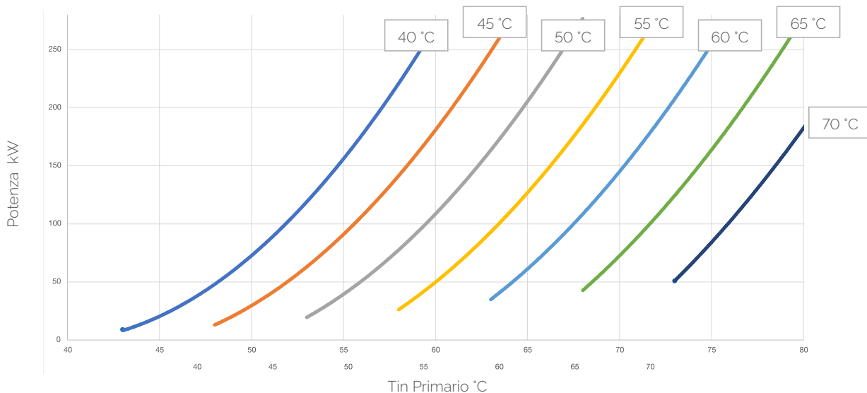
AQUAFAST 70/300 \Delta T=20^{\circ}\text{C}
