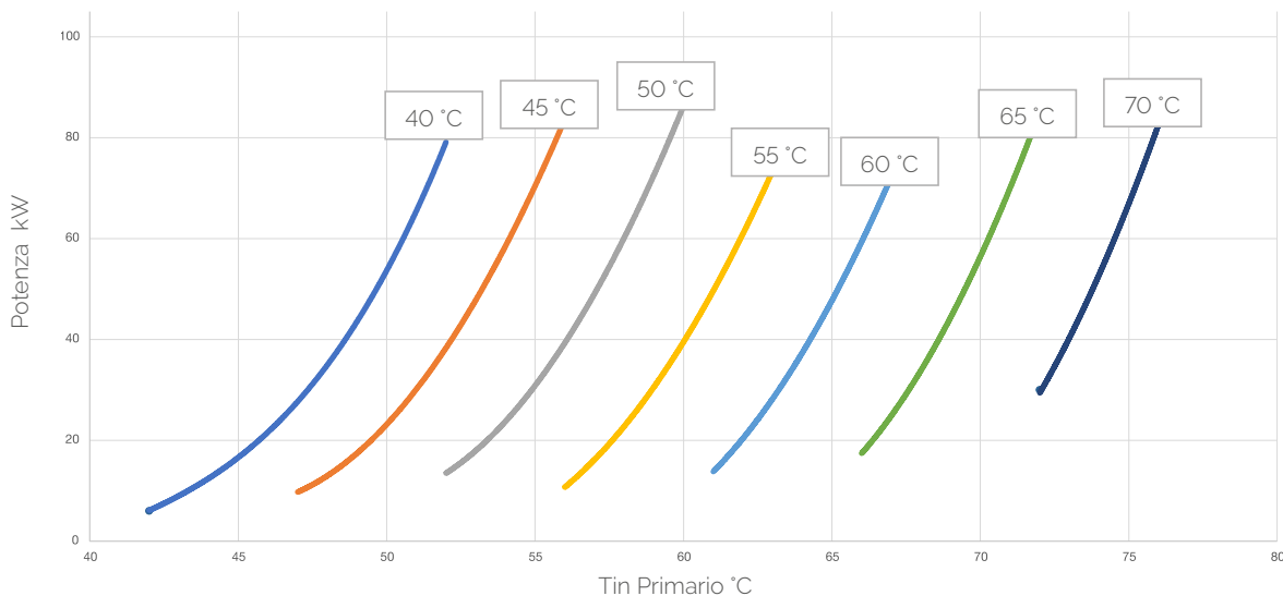
AQUAFAST 25/100 \Delta T=20^{\circ}\text{C}
