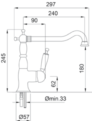
OXFORD Monocomando monoforo lavello canna tubo girevole con flex inox Single hole sink mixer swivel tube spout with flex
