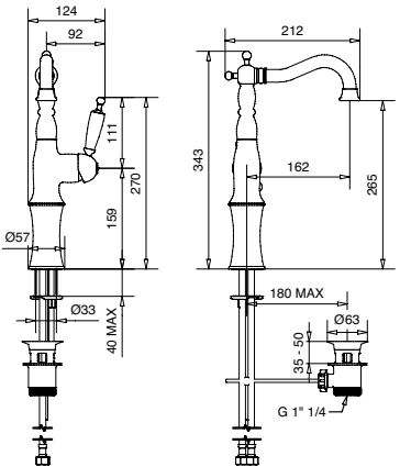
Monocomando lavabo modello alto scarico automatico 1"1/4 con flex inox Single hole basin mixer high model pop-up 1 "1/4 with flex
