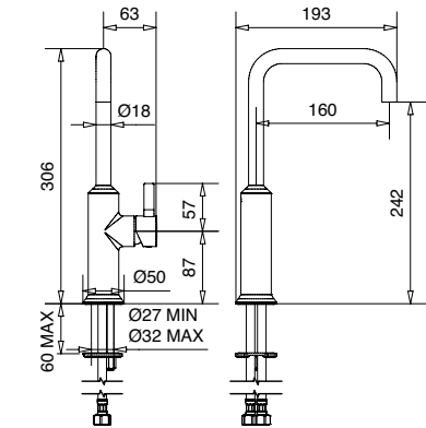
ORION Monocomando monoforo lavello canna girevole con flex inox Single hole sink mixer swivel spout with flex
