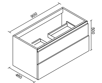
Base sospesa con 2 cassetti Wall cabinet with 2 drawers
