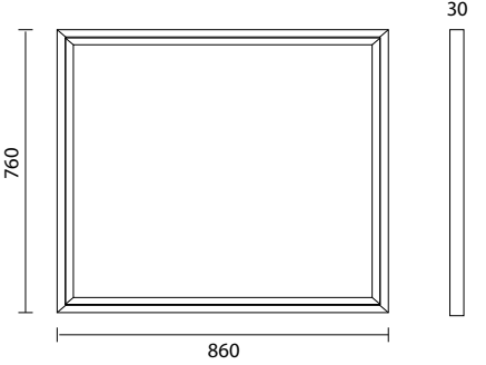
Specchiera illuminata con cornice LED Light mirror with LED frame
