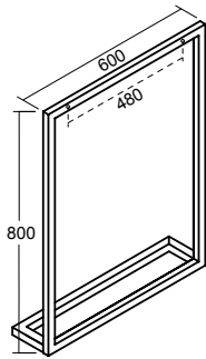
Specchio con mensola sagomata Mirror with shaped shelf
