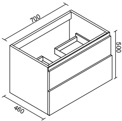
Base sospesa con 2 cassetti Wall cabinet with 2 drawers
