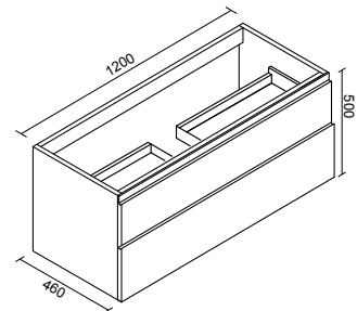
Base sospesa con 2 cassetti Wall cabinet with 2 drawers
