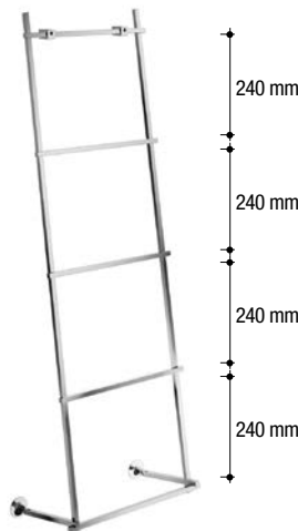
C480 Scaletta 4 barre Ladder with 4 bars L. 346 H. 1080 P. 210 mm
