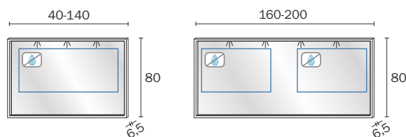
FRAME
